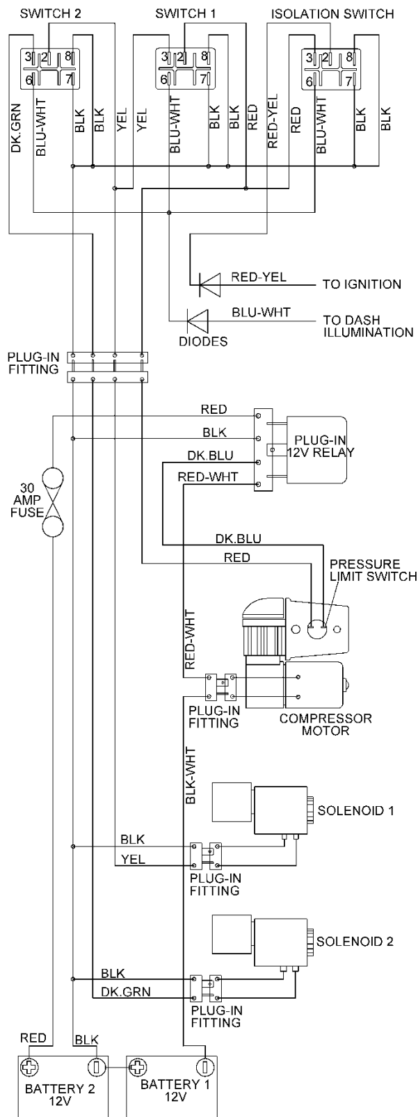
RDCKA24 24V VEHICLE LOOM
